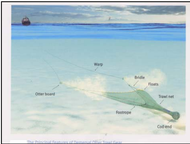
The Principal Features of Demersal Otter Trawl Gear
